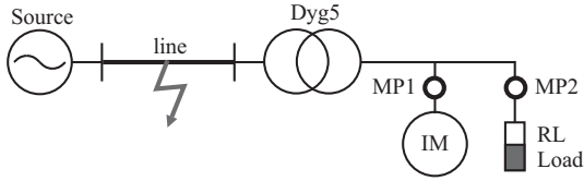
Fig. 4. Radial network example during an upstream fault.
