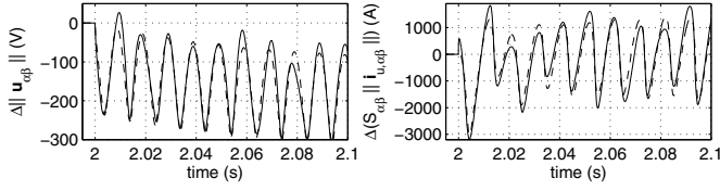
Fig. 8. Time responses obtained by the generalized resistance sign-based method for the upstream phase a -to-phase b fault (Fig. 4-MP1): perturbed supply voltage (solid line) and nominal supply voltage (dashed line).
