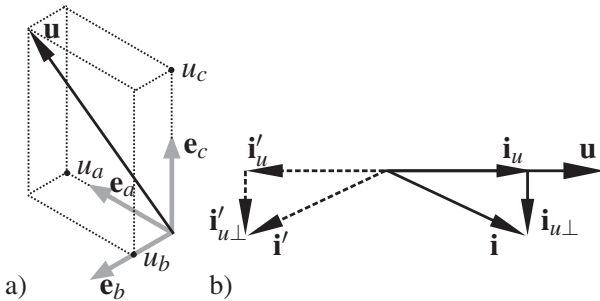
Fig. 1. Graphic presentation of the voltage vector (a), and orthogonal projections of the current vector (b) considering orientation of the active current vector (b - dashed case).
