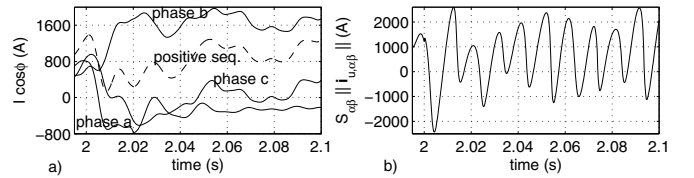
Fig. 7. Time responses obtained by the active current-based method for the upstream phase a -to-phase b fault (Fig. 4-MP1) - perturbed supply voltage: phasor-based method (a) and generalized method (b).
