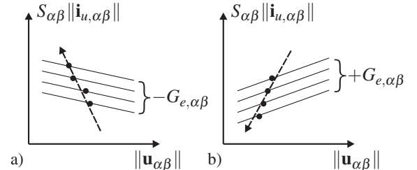
Fig. 3. Characteristic (\|\mathbf{u}_{\alpha\beta}(t)\|, S_{\alpha\beta} \|\mathbf{i}_{u,\alpha\beta}(t)\|) : downstream event (a), and upstream event (b).
