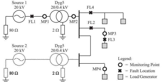
Fig. 9. Testing-network for numerical simulations of voltage sags: radial network (solid line) and non-radial network (solid and dashed line).
