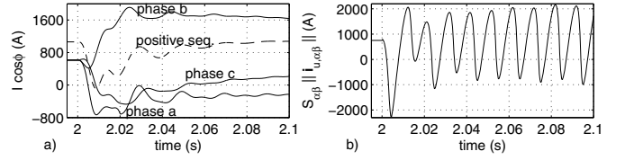
Fig. 6. Time responses obtained by the active current-based method for the upstream phase a -to-phase b fault (Fig. 4-MP1): phasor-based method (a) and generalized method (b).
