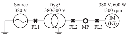
Fig. 11. Laboratory set-up for generation of voltage sags.
