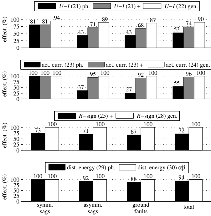
Fig. 10. Effectiveness of the discussed methods for voltage sag source detection, where (·) is equation number.
