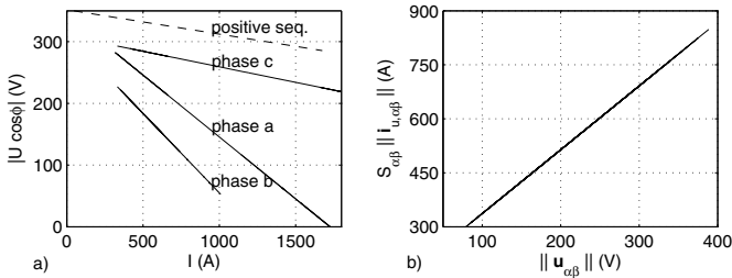
Fig. 5. Trajectories obtained by the voltage-current method for the upstream phase a -to-phase b fault (Fig. 4-MP1): phasor-based method (a) and generalized method (b).
