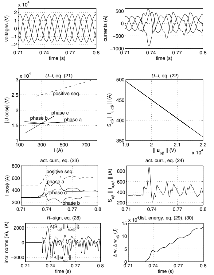
Fig. 12. Field testing results for the downstream transformer energizing.
